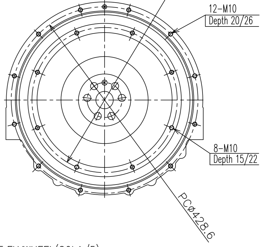
DETAIL OF FLYWHEEL(SCL1/5)
