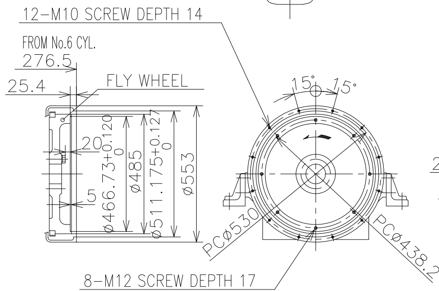
DETAIL OF REAR P.T.O. (S:1/15)
