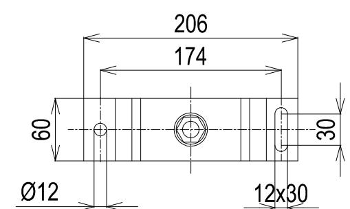
DETAIL OF MOUNTING BLOCK
