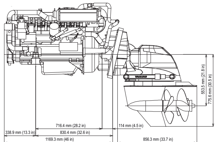
6LPA-STP2/C with ZT370r (Not to be used for engine installation)
