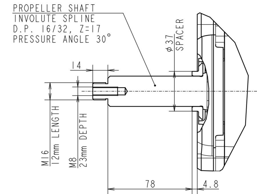
PROPELLER SHAFT (NOT TO SCALE)
