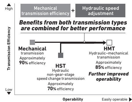
HMT (Hydro-Mechanical Transmission)
