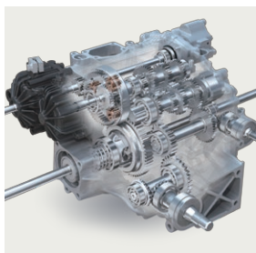
HMT (Hydro-Mechanical Transmission)
