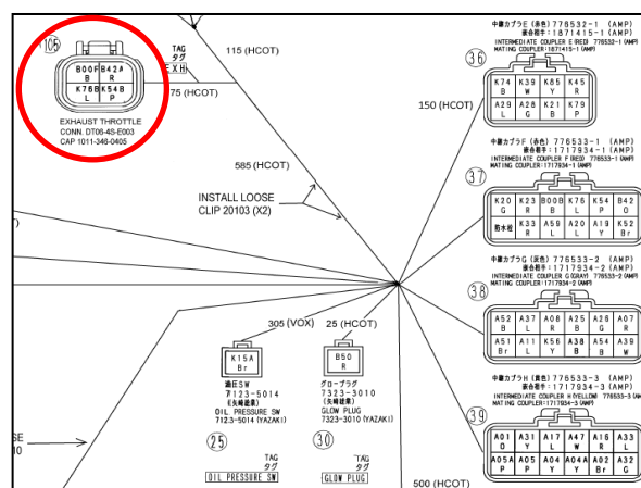
Picture 2. Main Harness
